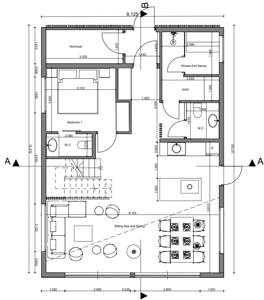
0. Groundfloor 1:100
