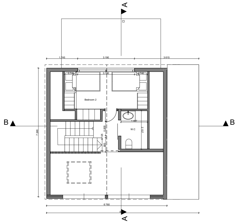
1. First Floor 1:100
