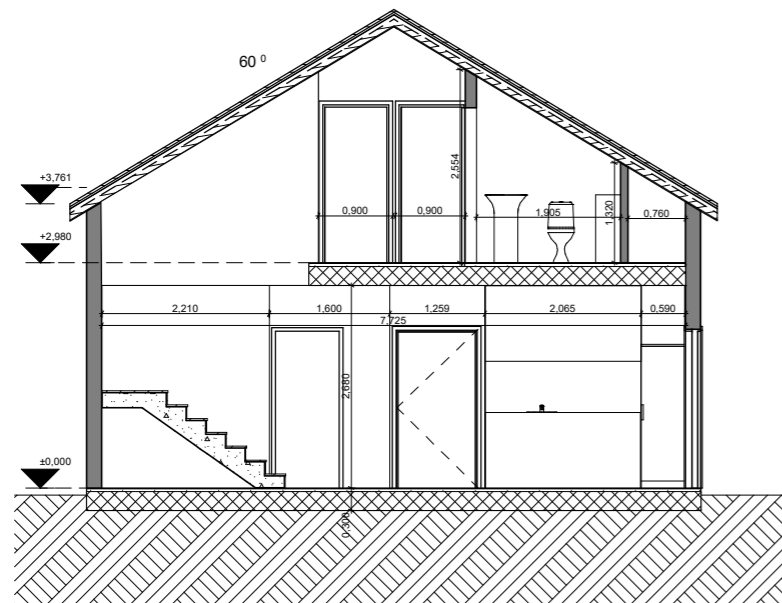
Section A 1:100
