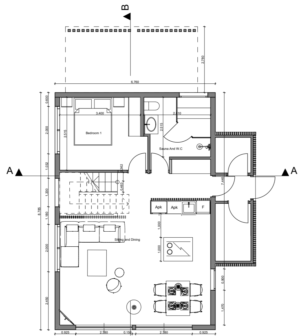
0. Groundfloor 1:100
