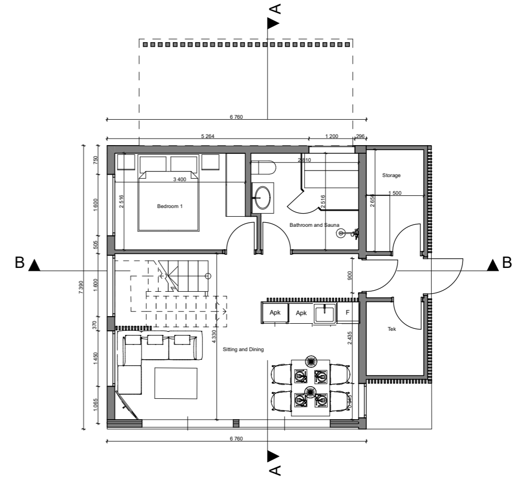
0. Groundfloor 1:100
