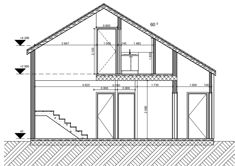
Section AA 1:100
