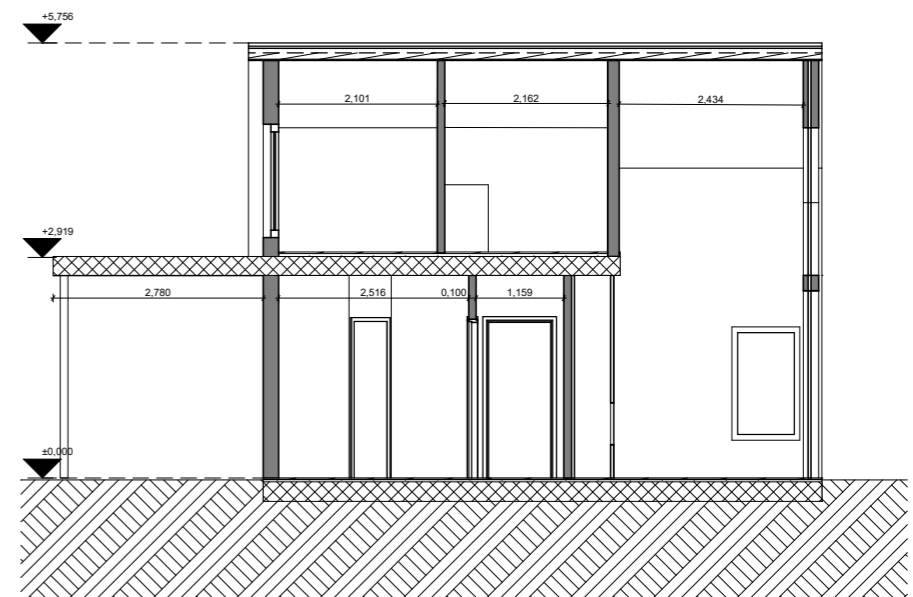
Section AA 1:100
