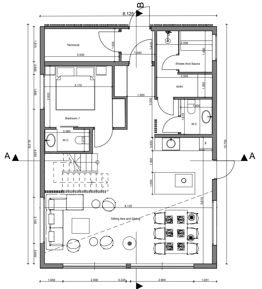
0. Groundfloor 1:100
